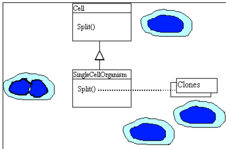
Figure 5: Object Diagram for Prototyping Cell Division Example
